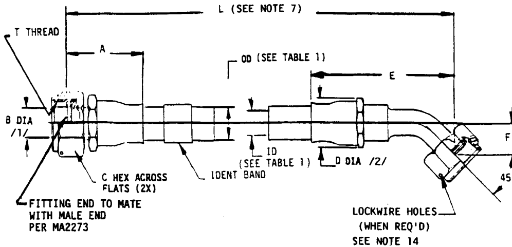
FIGURE 1 - DETAIL OF HOSE ASSEMBLY
