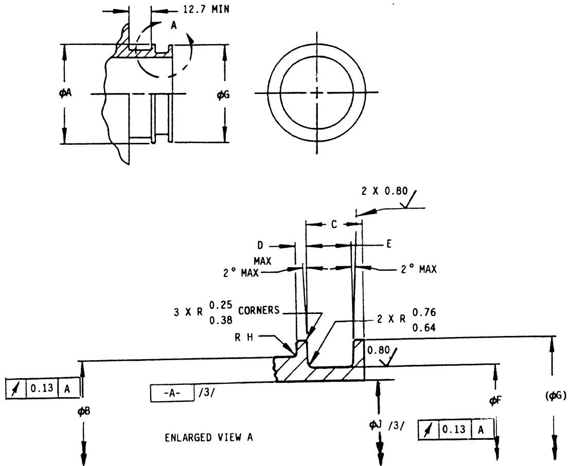
FIGURE 1 - FERRULE END
