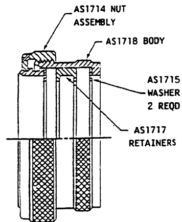
FIGURE 4 - AS1712 COUPLING SUBASSEMBLY /11/
