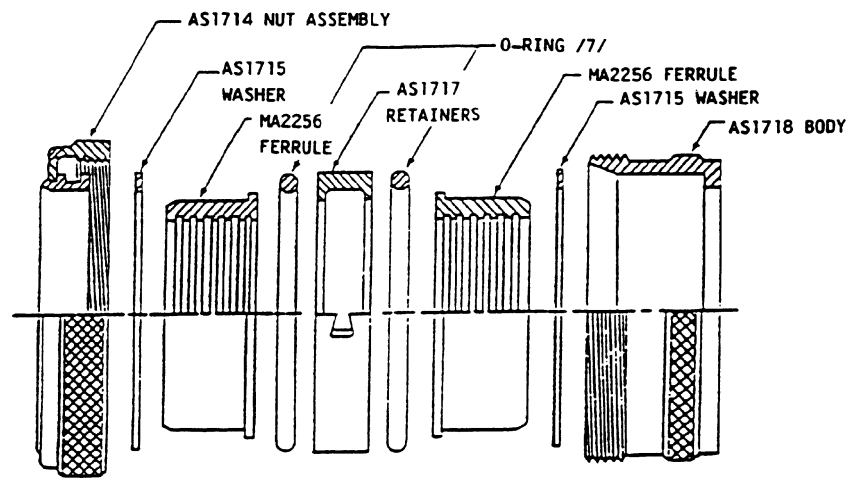
FIGURE 3 - EXPLODED VIEW FULL COUPLING /10/
