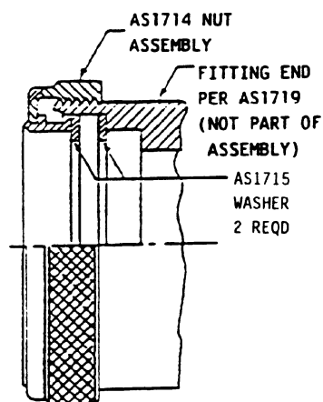
FIGURE 5 - AS1713 HALF COUPLING SUBASSEMBLY /12/
