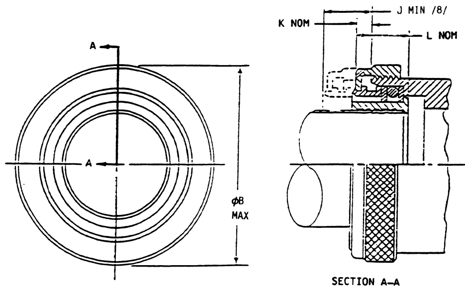
FIGURE 2 - HALF COUPLING
