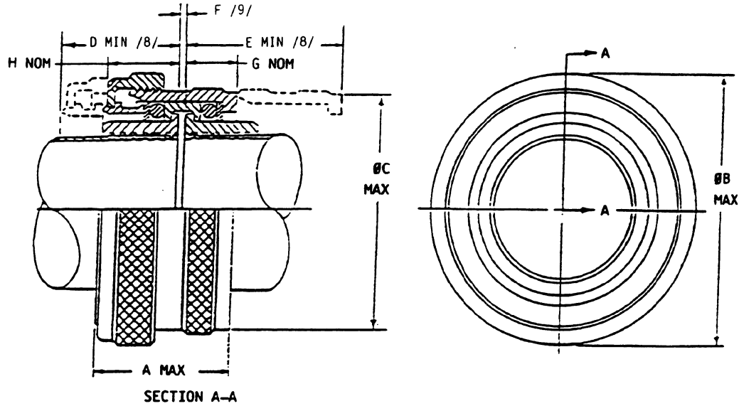
FIGURE 1 - FULL COUPLING
