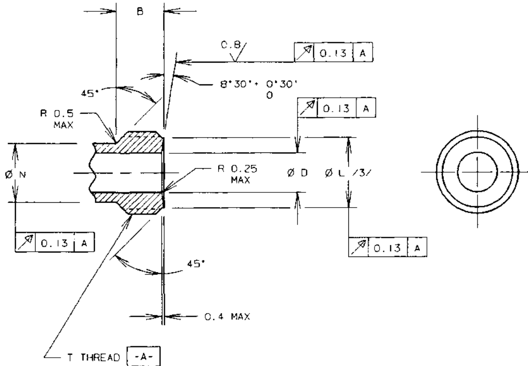
FIGURE 1 - FITTING END DESIGN, STYLE A
