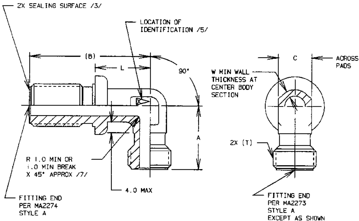
FIGURE 1 - ELBOW, 90°, BULKHEAD BEAM SEAL
