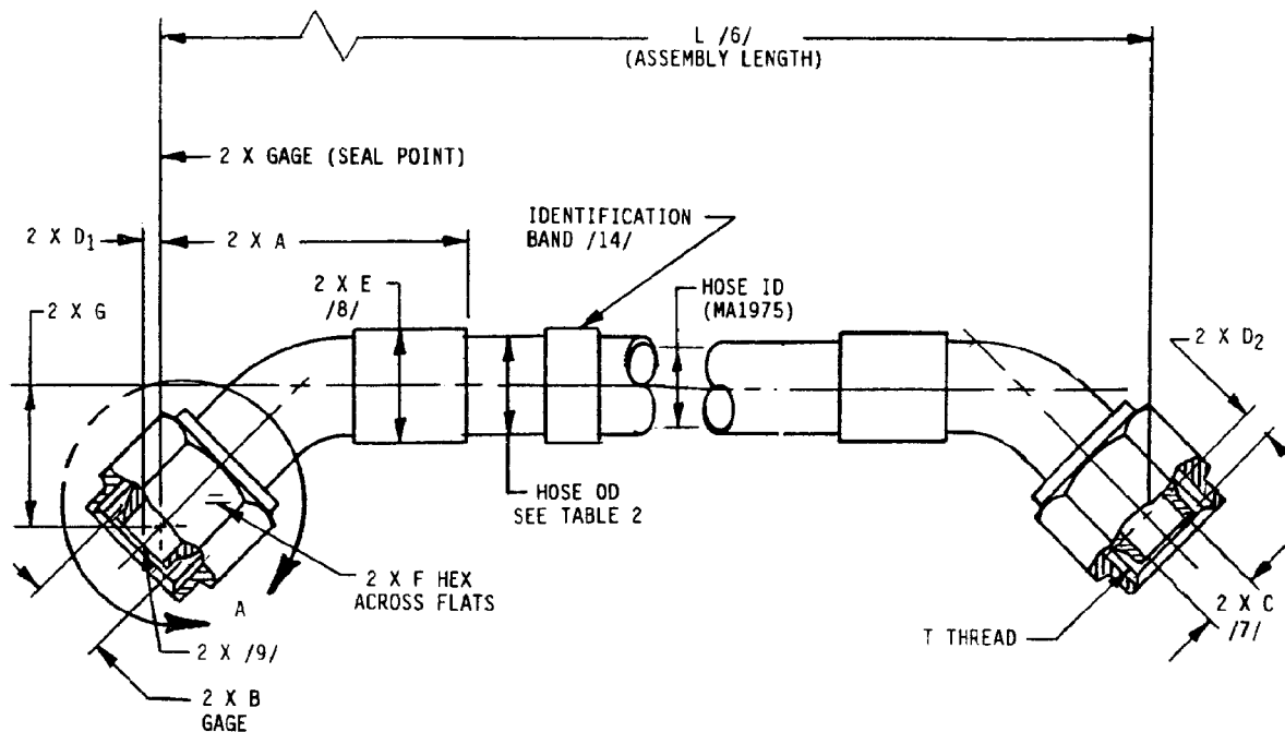
FIGURE 1 - FLARELESS HOSE ASSEMBLY 45° ELBOW TO 45° ELBOW
