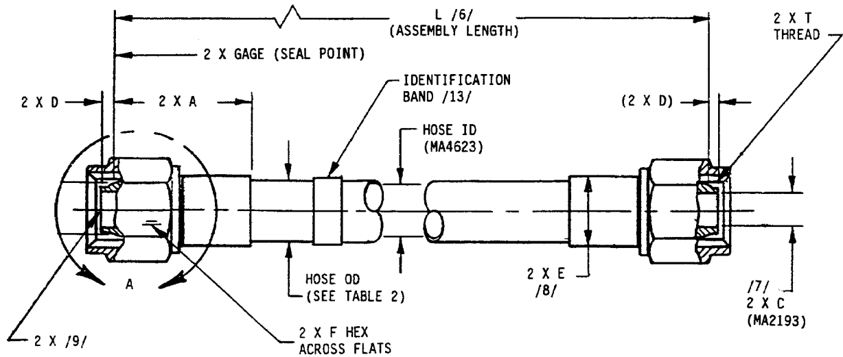
FIGURE 1 - FLARELESS HOSE ASSEMBLY, STRAIGHT TO STRAIGHT
