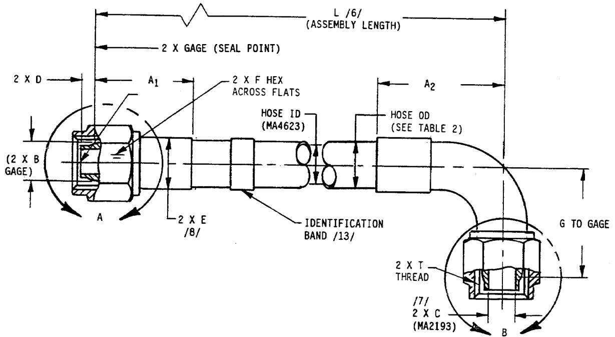
FIGURE 1 - FLARELESS HOSE ASSEMBLY STRAIGHT TO 45° ELBOW
