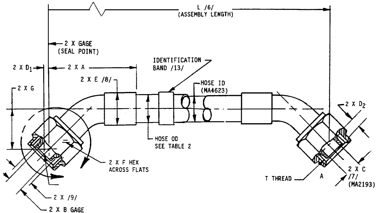
FIGURE 1 - FLARELESS HOSE ASSEMBLY 45° TO 45° ELBOW
