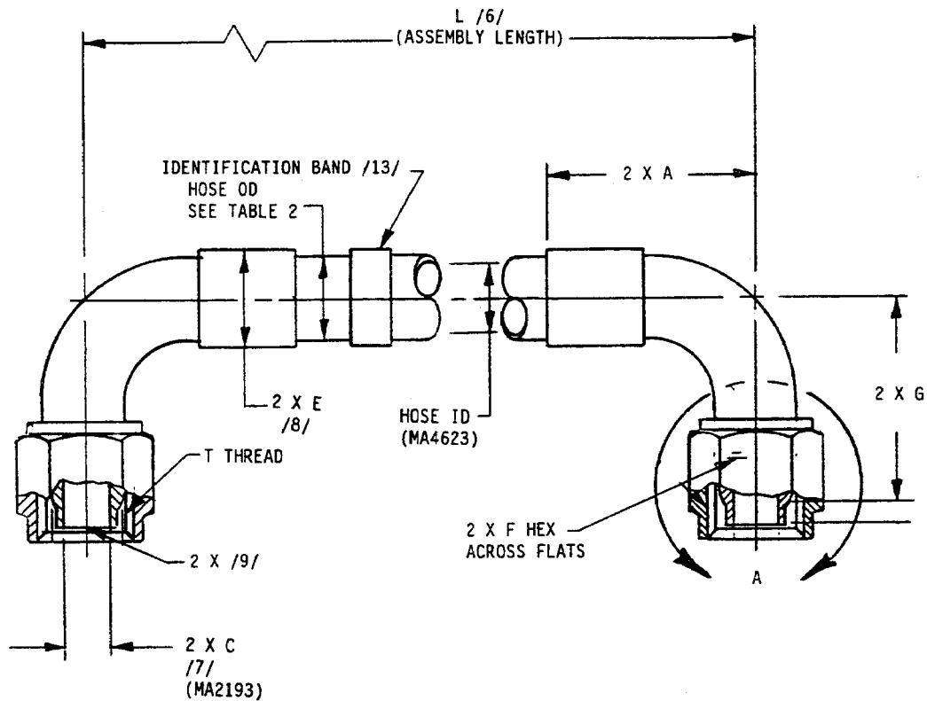
FIGURE 1 - FLARELESS HOSE ASSEMBLY 90° TO 90° ELBOW
