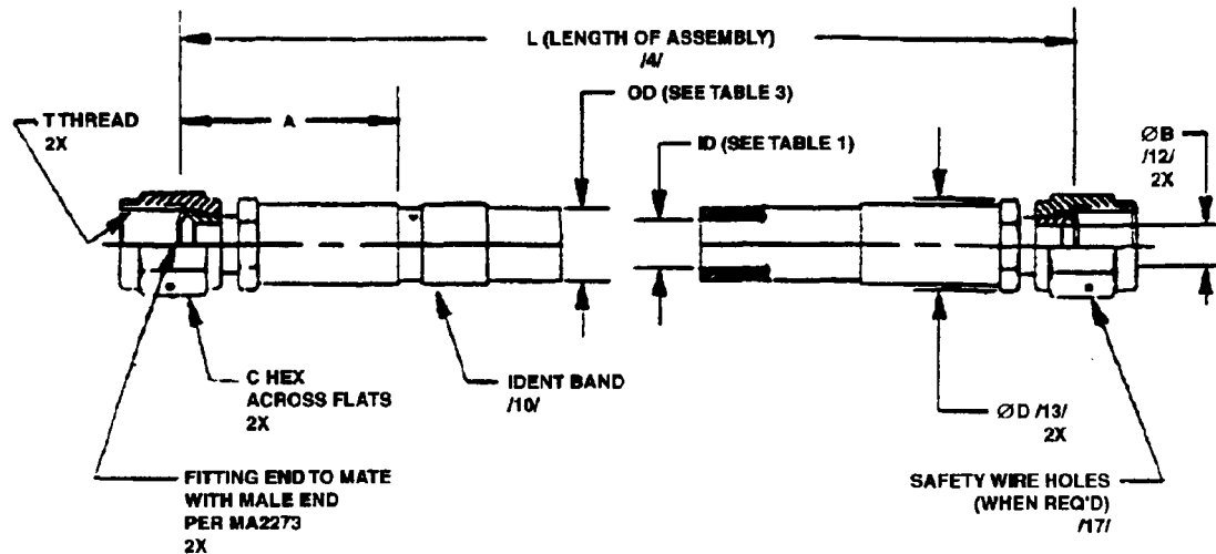
FIGURE 1 - HOSE ASSEMBLY
