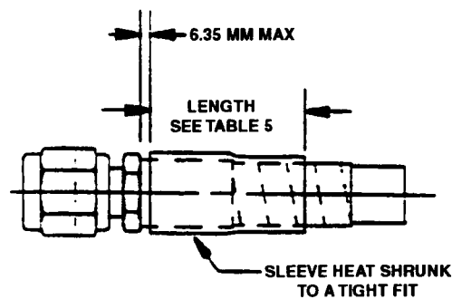
FIGURE 2 - HEAT SHRINKABLE SLEEVES REQUIRED FOR COIL AND TUBULAR ABRASION SLEEVES /16/ AND /17/
