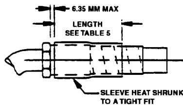
FIGURE 2 - HEAT SHRINKABLE SLEEVES REQUIRED FOR COIL AND TUBULAR ABRASION SLEEVES /16/ AND /7/
