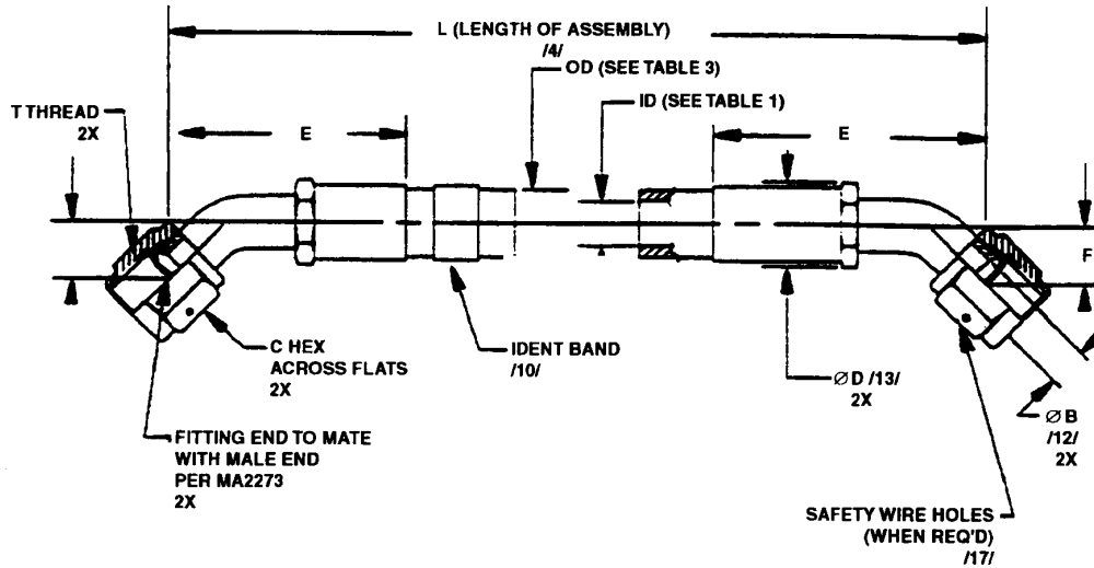
FIGURE 1 - HOSE ASSEMBLY
