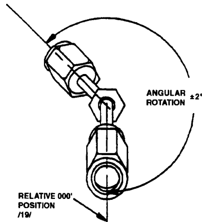
FIGURE 3 - FITTING ANGULAR ORIENTATION
