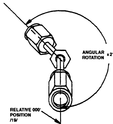
FIGURE 3 - FITTING ANGULAR ORIENTATION
