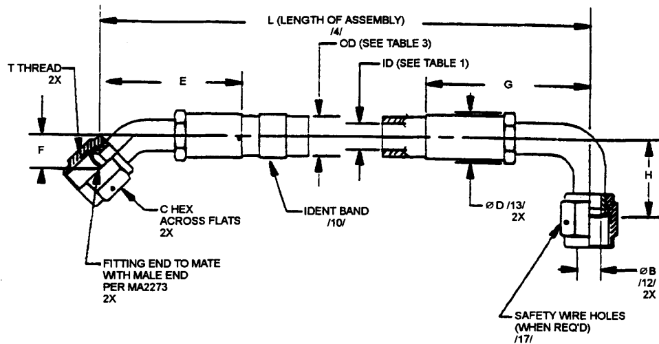
FIGURE 1 - HOSE ASSEMBLY
