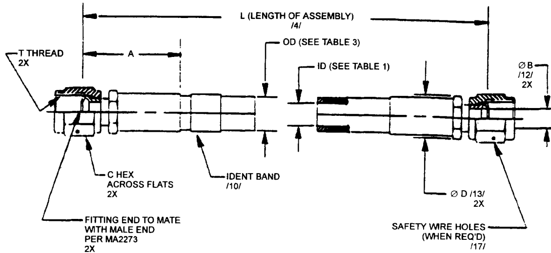
FIGURE 1 - HOSE ASSEMBLY
