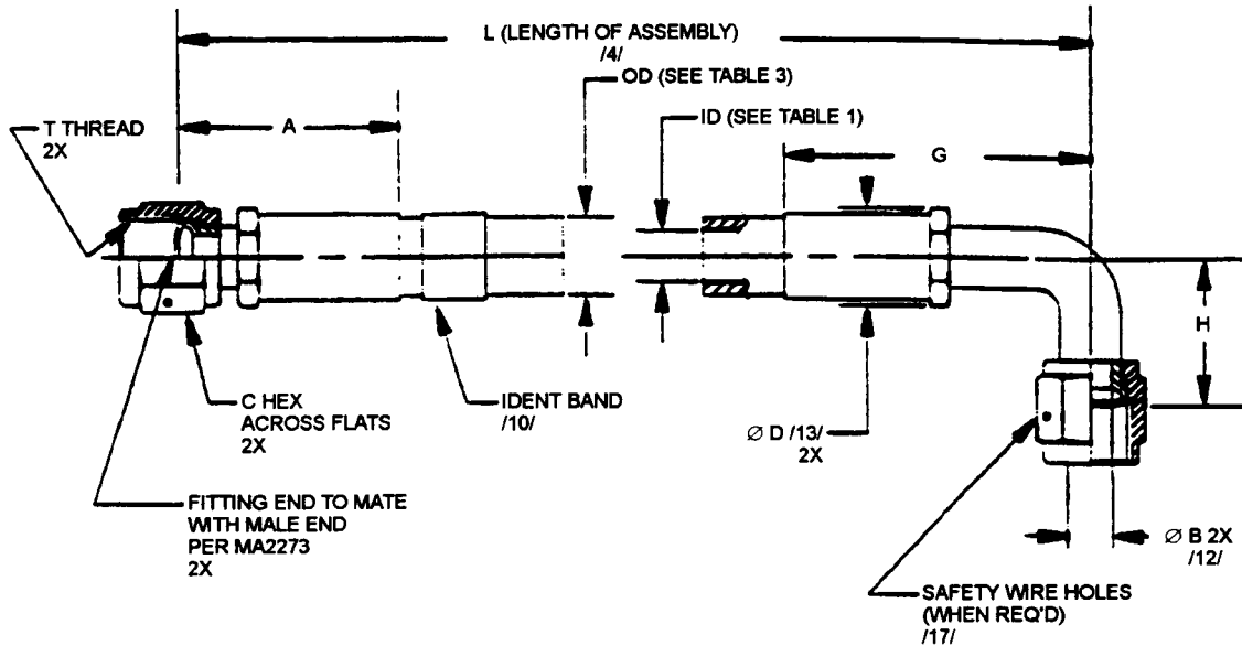
FIGURE 1 - HOSE ASSEMBLY
