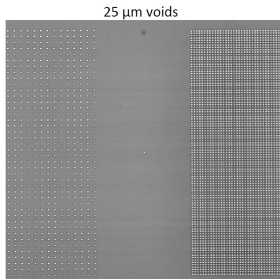
Figure 5 IR Microscopy Image of 25- \mu\text{m} Wide, 1200-nm Thick Voids
