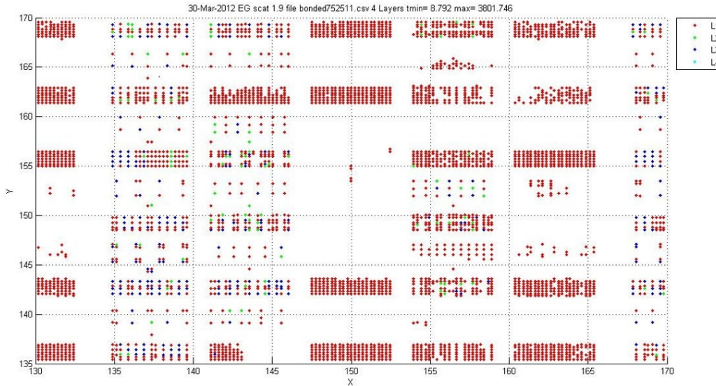
Figure 4 Result of IR Interferometry Scanning of One Die on a Bond Void Specimen Wafer
