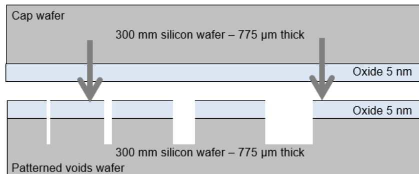
Figure 1 Schematic Diagram Showing the Etched Wells Used to Produce Voids at the Bonded Interface Between Two Wafers
