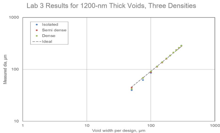
Figure 6 Plot Showing Lab 3 Void Size Measurement Results for 1200-nm Thick Voids of Three Densities
