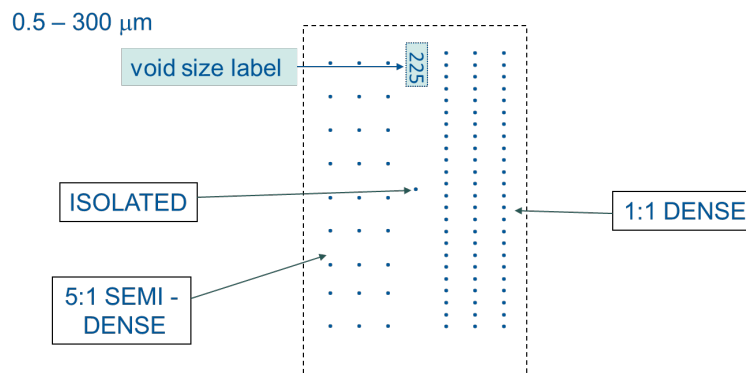
Figure 3 Details of the Arrangement of Artificial Voids at Different Densities
