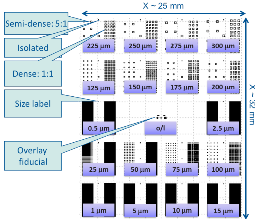
Figure 2 Layout of the Voids of Different Sizes and Densities in Die-Sized Arrays
