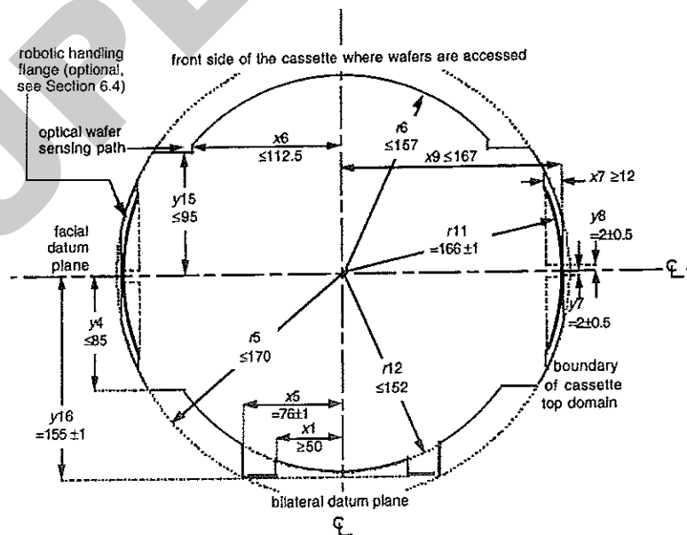
Figure 2 Cassette Top Domain
