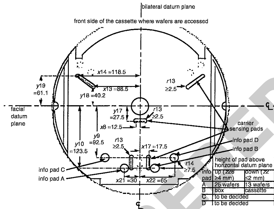
Figure 5 Carrier Sensing Pads in Bottom View
