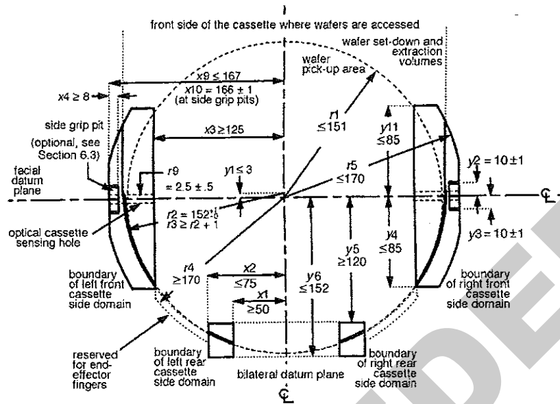
Figure 1 Cassette Side Domains
