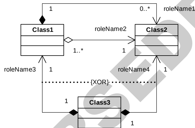
Figure 1 Association Notation
