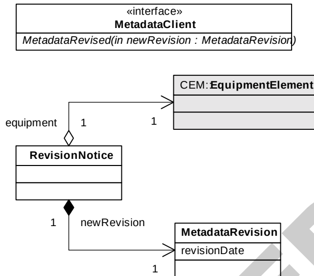
Figure 6 Metadata Client Interface
