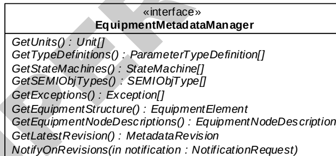
Figure 3 Interface for Accessing Equipment Metadata
