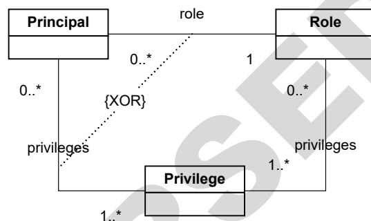
Figure 6 Abstract Model of ACL
