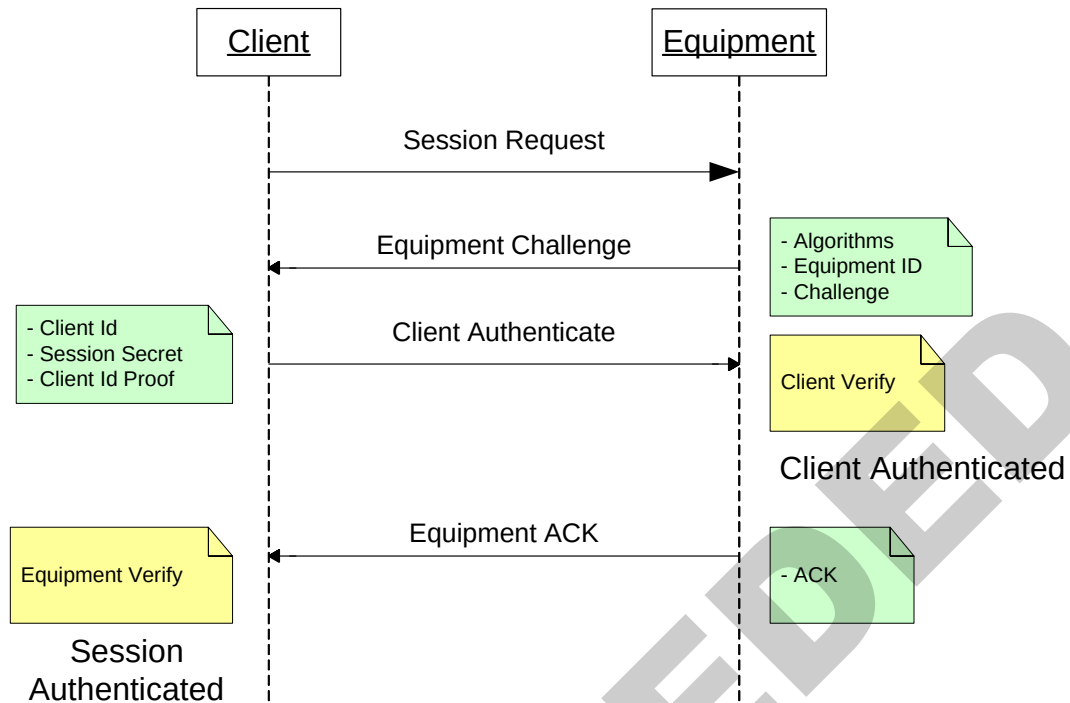
Figure 5 Authentication Message Flow
