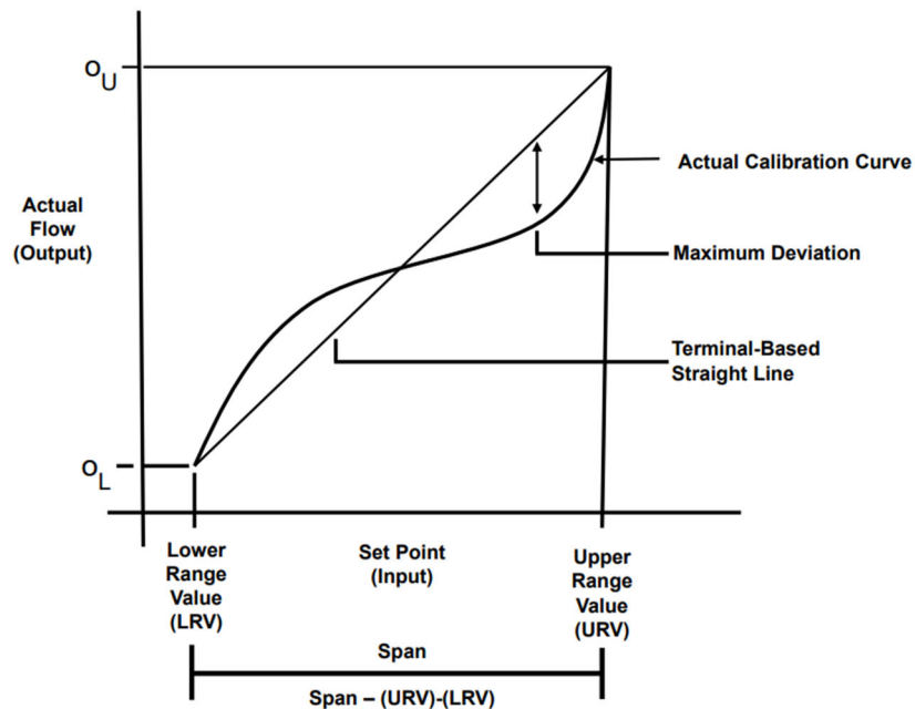
Figure 1 Terminal-Based Linearity of a Mass Flow Controller
