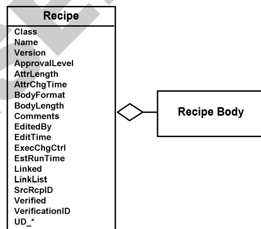
Figure 3.2 Recipe Supertype
