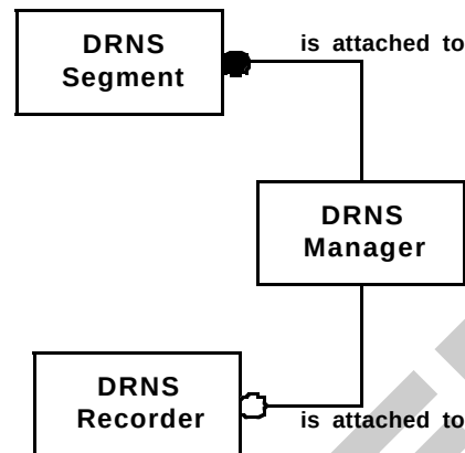
Figure 5.8 The Attachment Relationship
