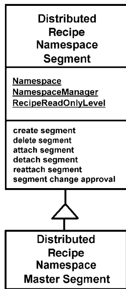
Figure 5.3 Distributed Recipe Namespace Segment
