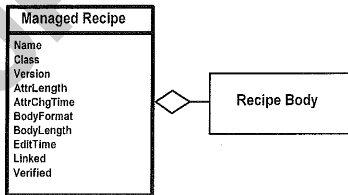
Figure 3.6 Object Model for Minimal Managed Recipe
