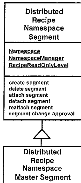
Figure 5.3 Distributed Recipe Namespace Segment
