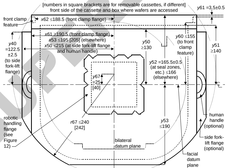
Figure 7 Top View of Front-Opening Box
