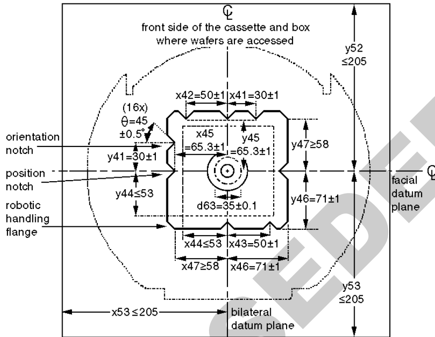
Figure 2 Rear View of Bottom-Opening Box
