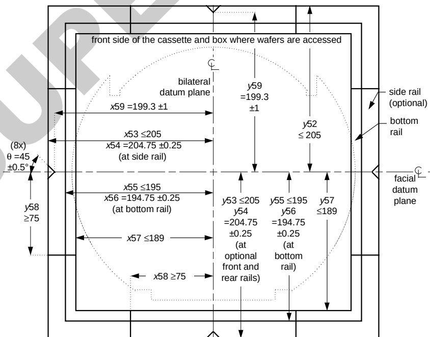
Figure 3 Top View of Bottom-Opening Box
