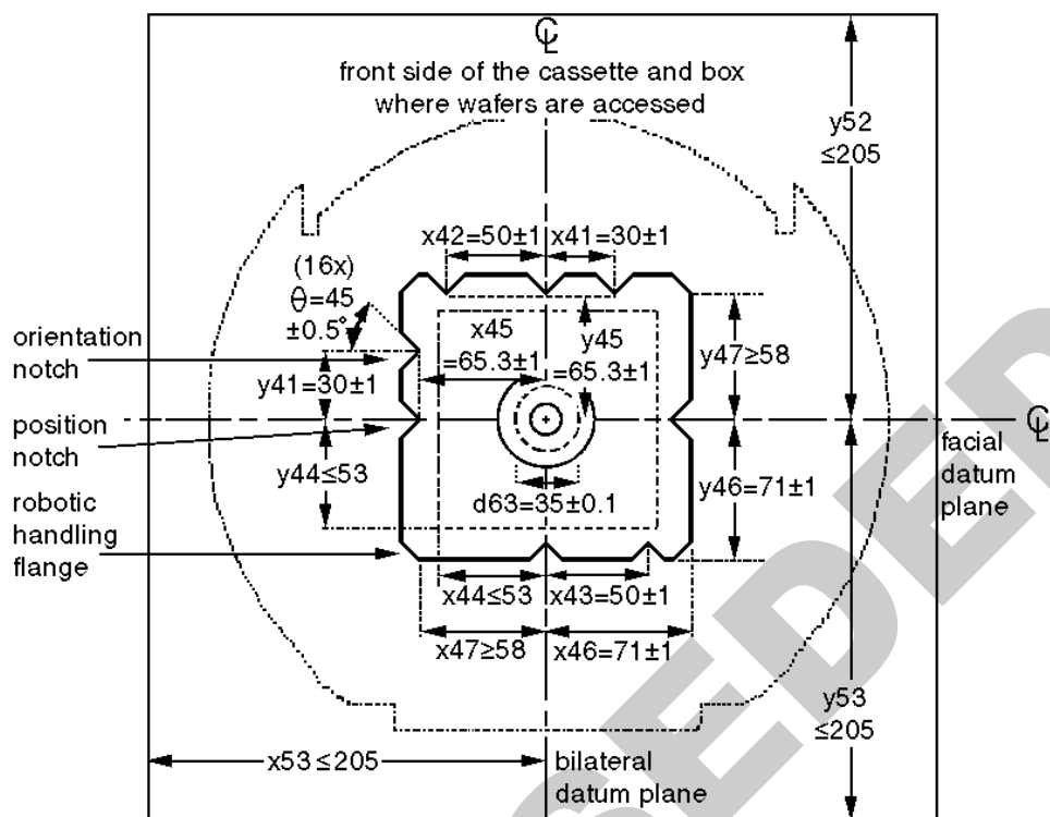
Figure 3 Top View of Bottom-Opening Box
