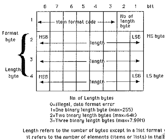
Figure 2 Item and List Header
