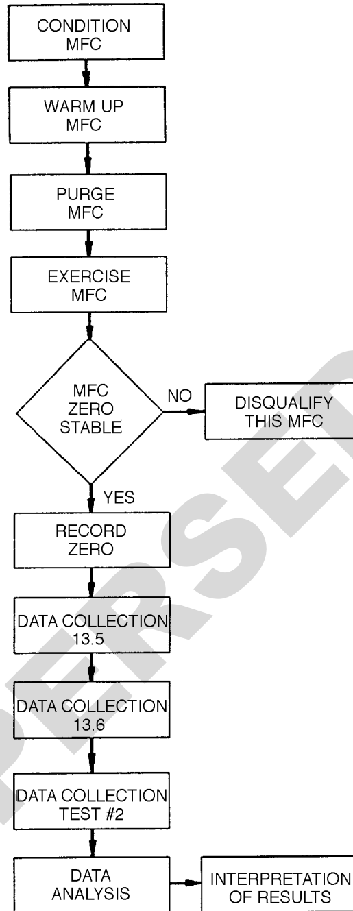
Figure 2 Test Flowchart
