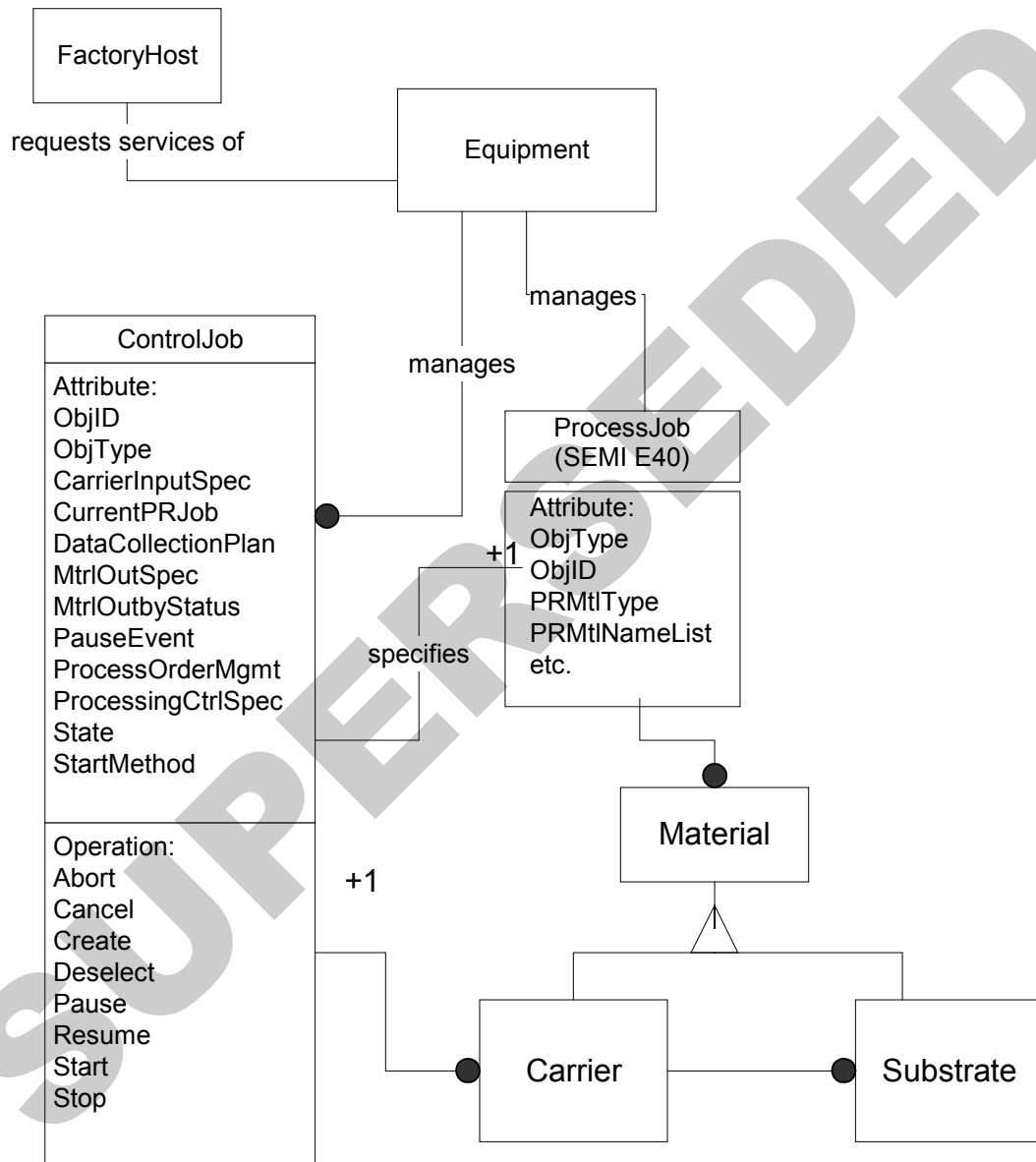
Figure 1 ControlJob Object Model
