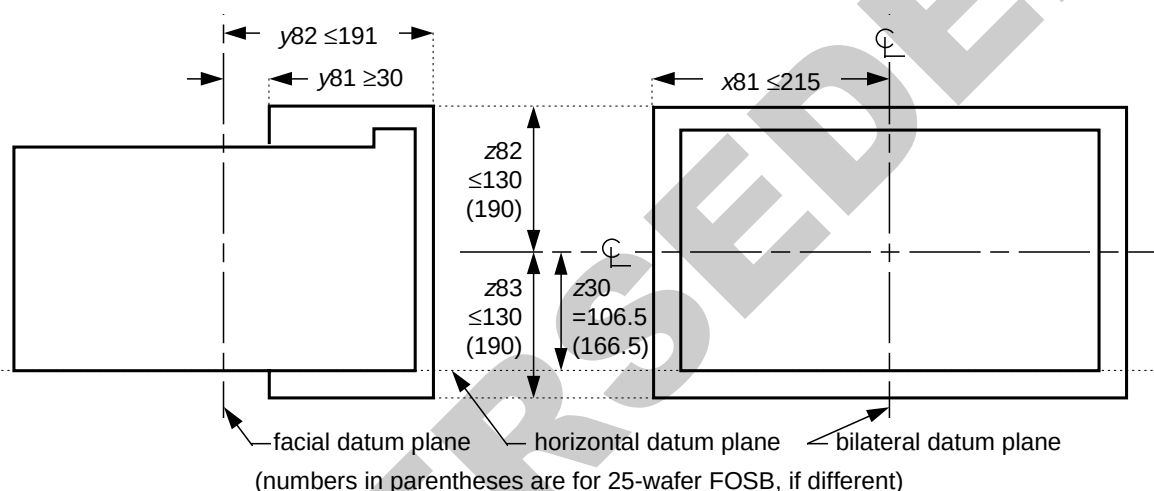
Figure 1 Manual Door Area
