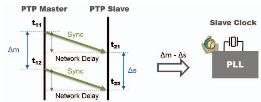
Figure 4 – Example of Frequency Control
