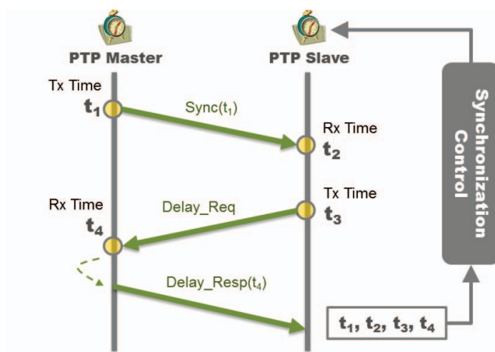
Figure 2 – Concept Diagram of the PTP Synchronization Control
