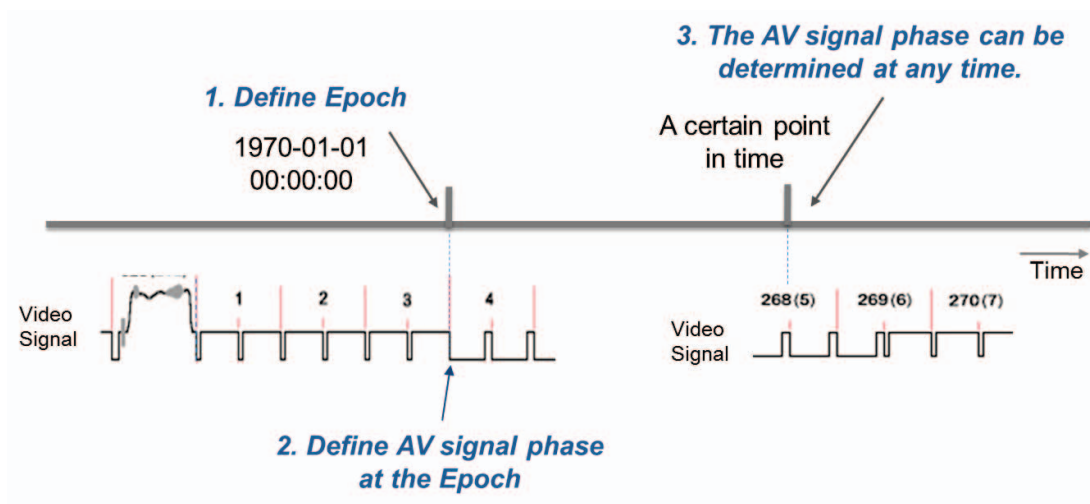
Figure 1 – Concept of the New Synchronization System
