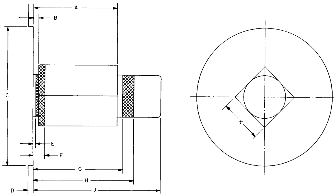
Figure 1 – 16-mm motion-picture camera spindles
