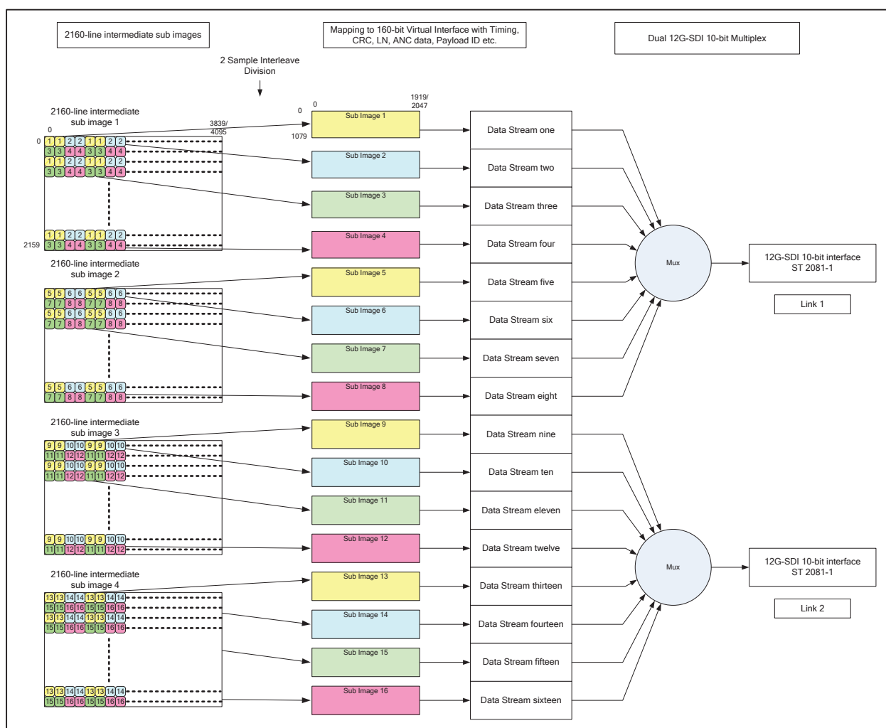
Figure 4 – 2 sample division of the four 2160-line intermediate sub images to sixteen 1080-line sub images, and mapping into a Dual-link 12G-SDI interface
