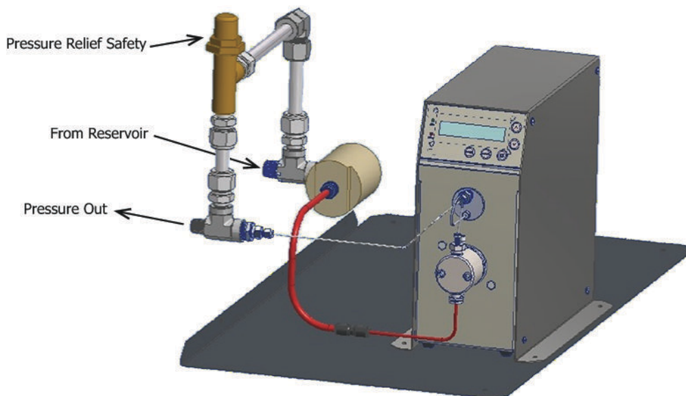
FIG. 2 Alternative Hydraulic and Power System
