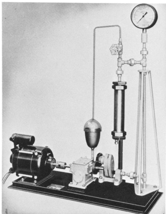
FIG. 3 Photograph of Apparatus
