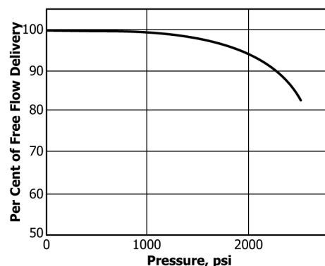
FIG. 4 Typical Pump Calibration Curve
