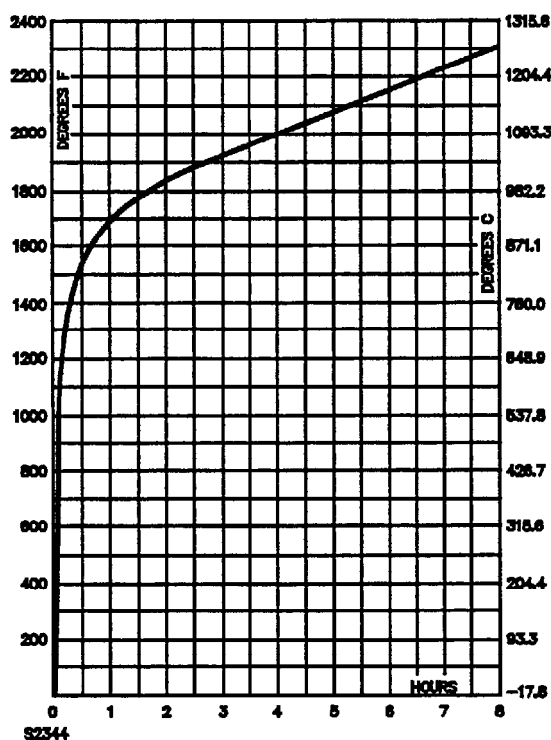
(DELETED) Figure 3.1 Time-temperature curve
