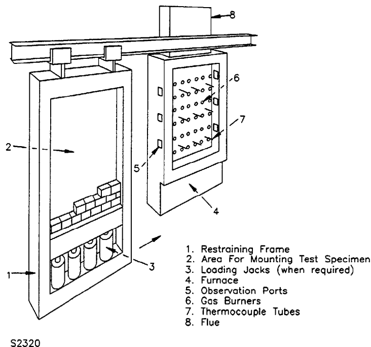
Figure 4.5.1 Test furnace
