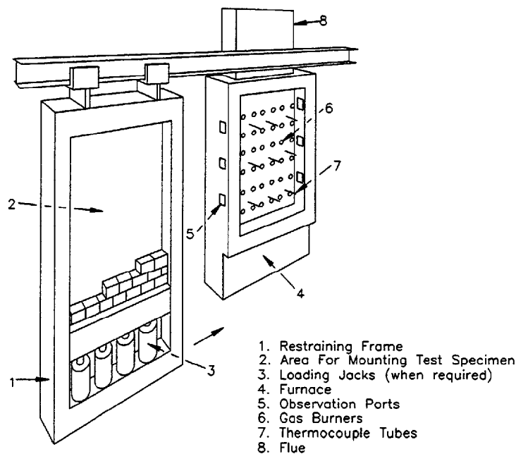
Figure 4.5.1 Test furnace
