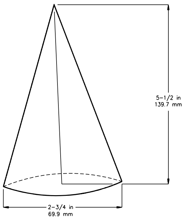
Figure 10.1 Cone probe
