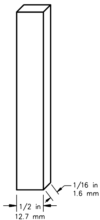
Figure 10.2 Bar probe
