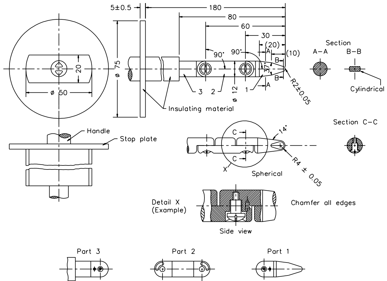
Figure 8.4 Articulate probe
