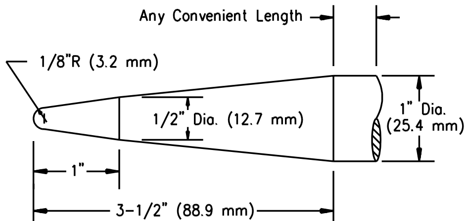
Figure 9.1 Probe for fan blades of air heaters
