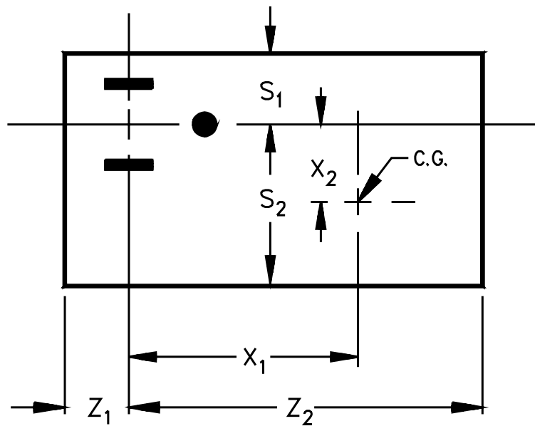
Figure 7.1 Dimensions of a plug-in product
