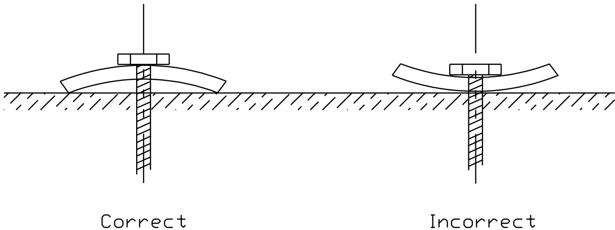
Figure 7.2 Orientation of spring washer
