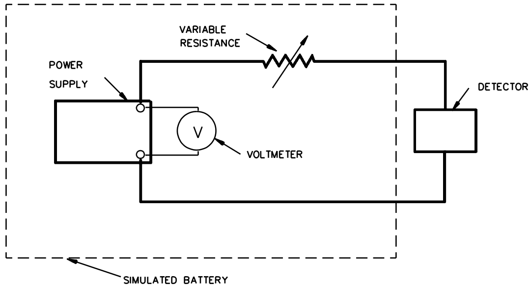
Figure 35.1 Test circuit
