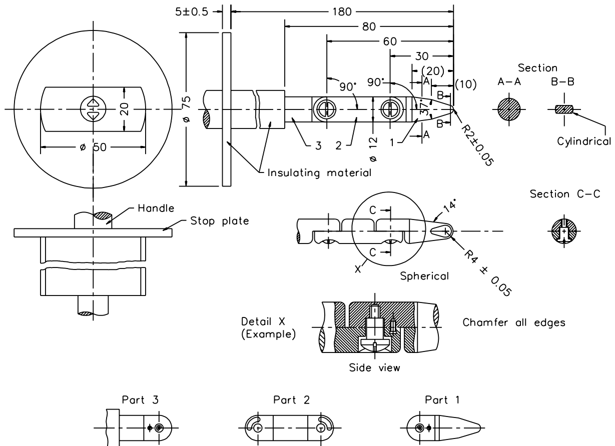
Figure 13.1 Articulate probe with web stop (Dimensions in mm)
