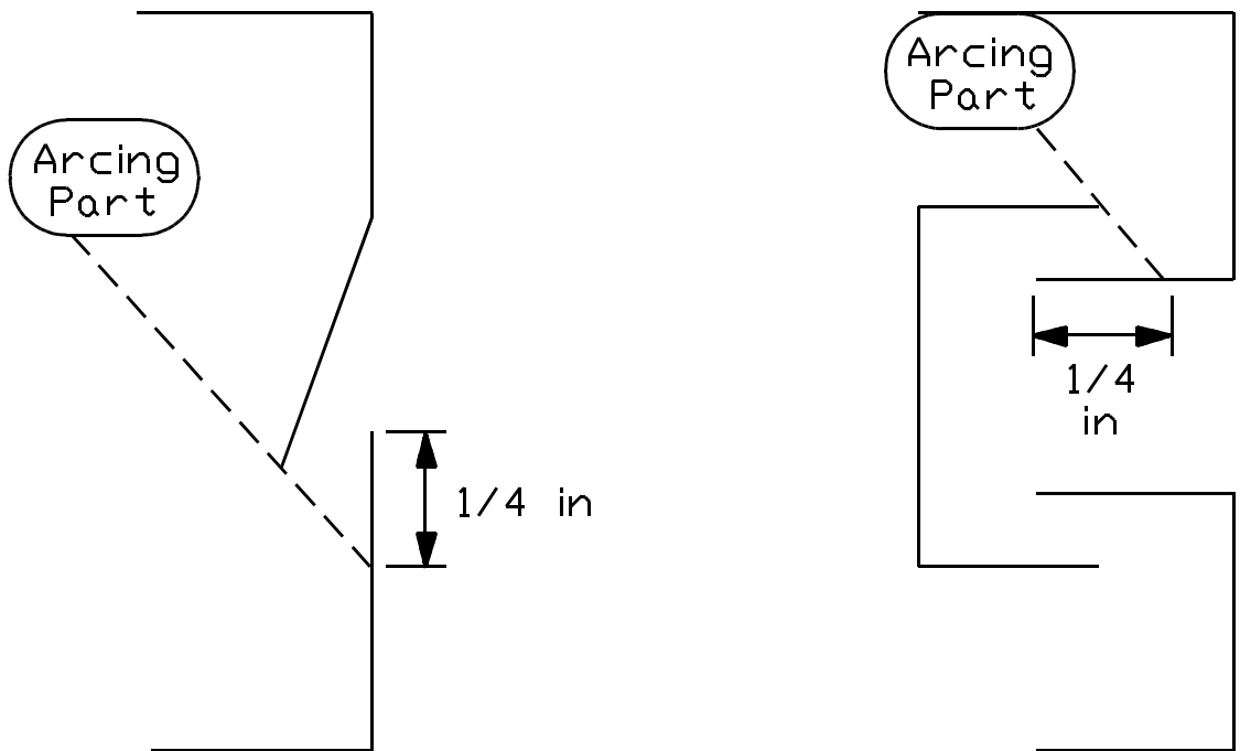
Figure 22.1 Barriers for ventilation openings
