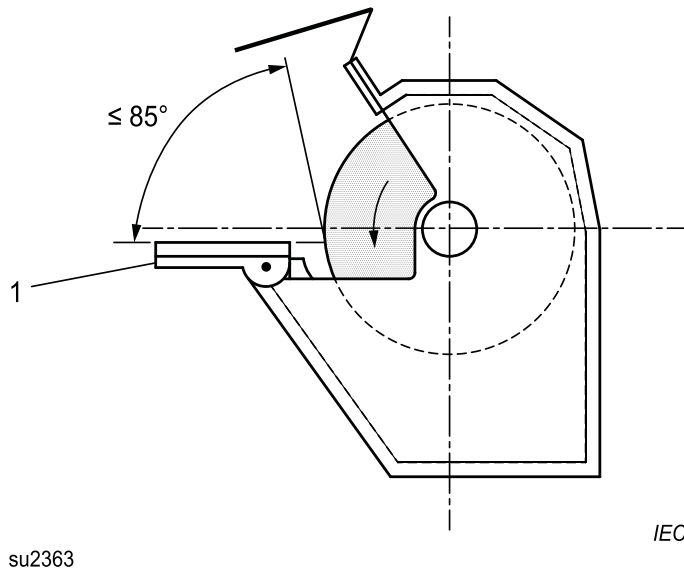
Figure 104 – Bench grinder with inclinable work rest
