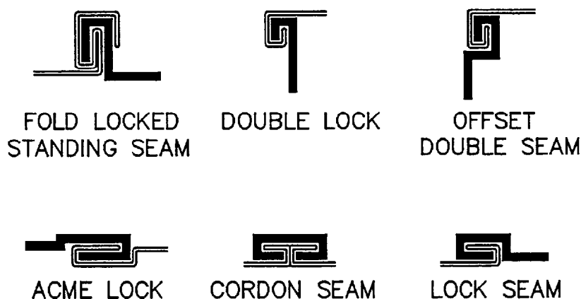
Figure 14.1 Types of acceptable lock-seams
