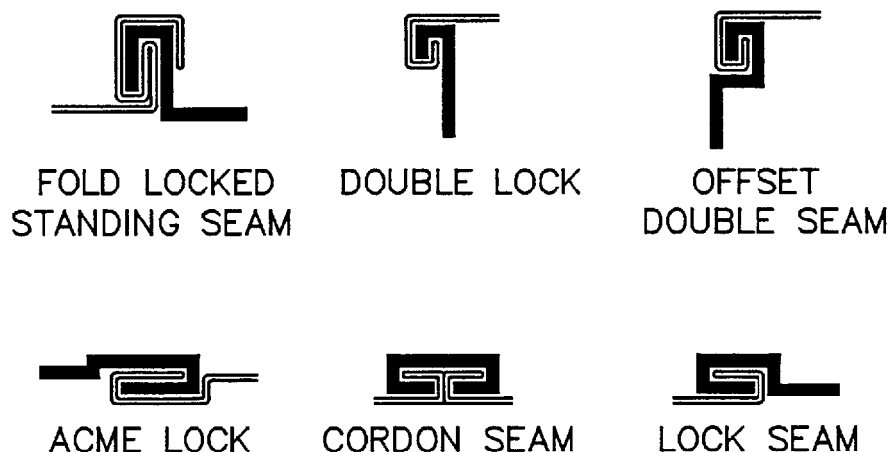
Figure 12.1 Types of acceptable lock-seams
