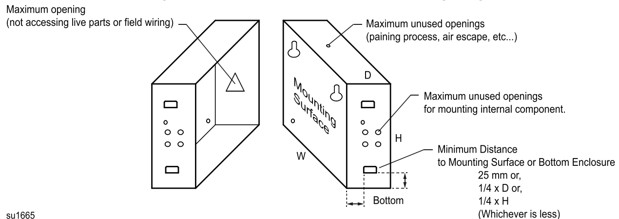
Figure 5.2 Examples of Shortest Distances from Enclosure Openings
