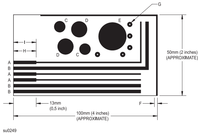
Figure 10.1 Typical test pattern coupon for bond strength, delamination, plating and conductive paste adhesion testing
