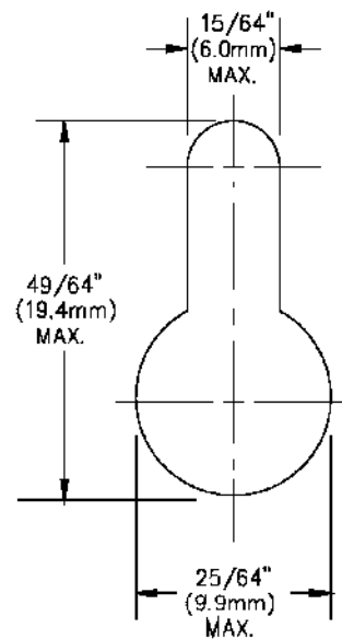
Figure 7.3 Keyhole slot
