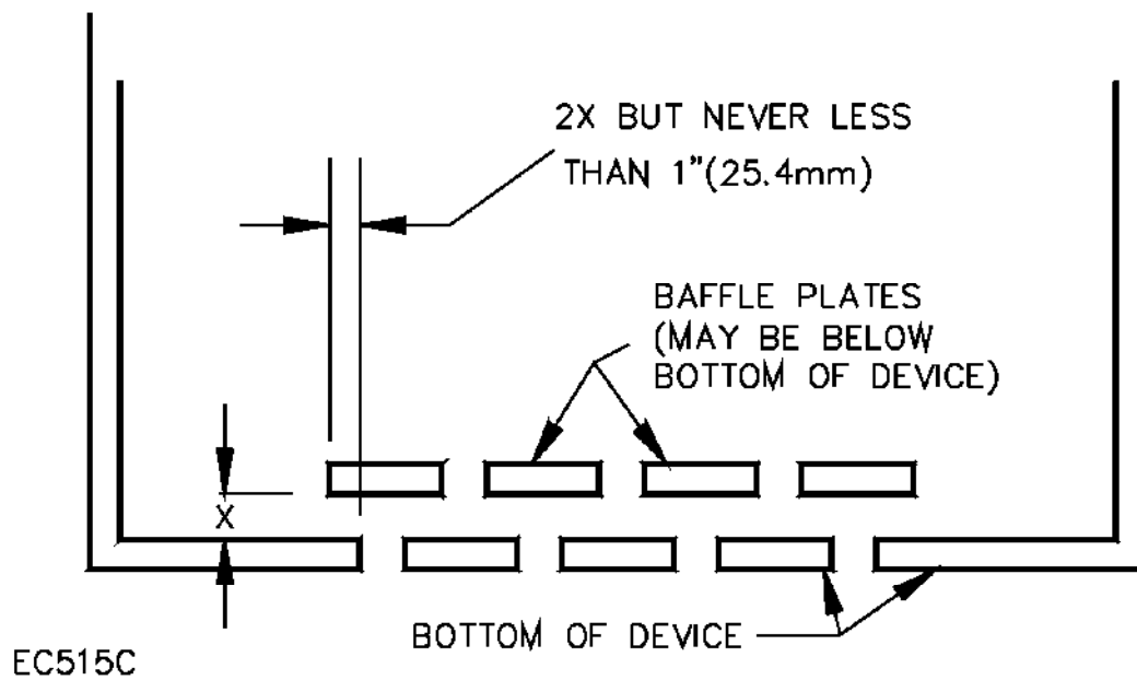
Figure 7.2 Bottom surface openings of enclosures
