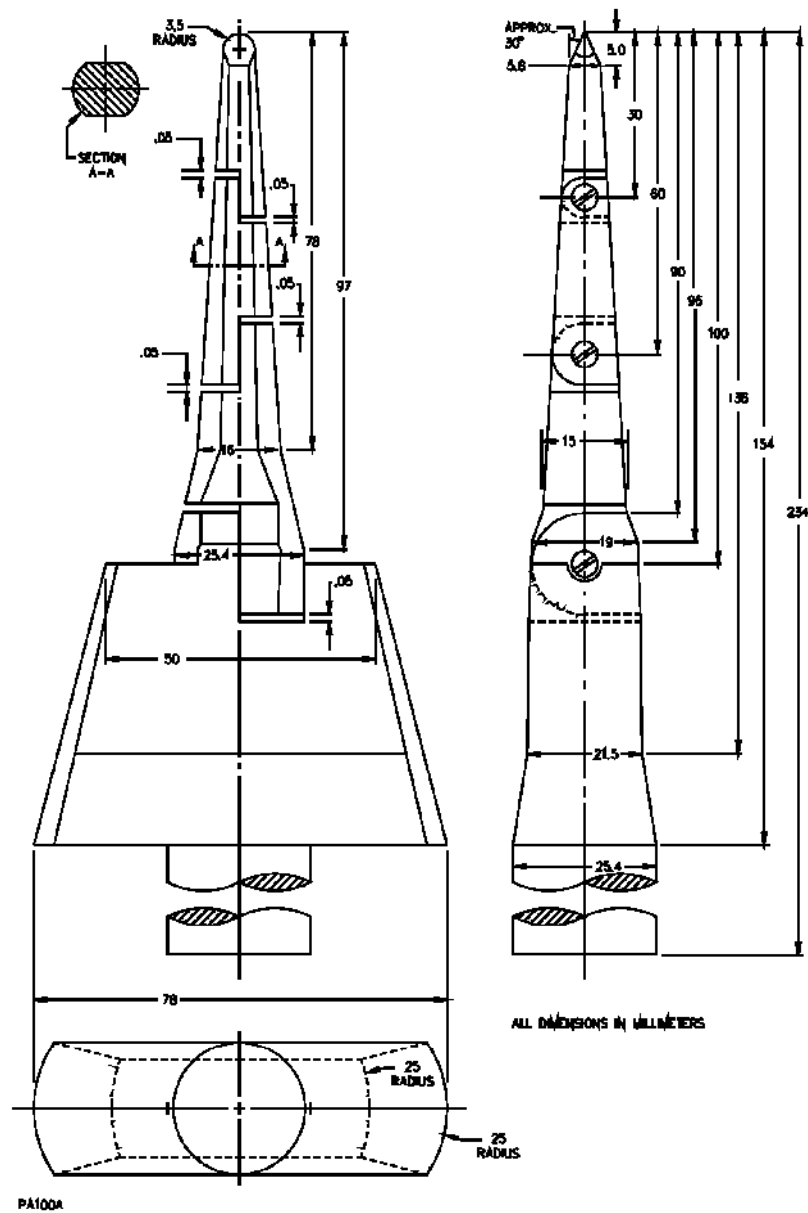
Figure 7.1 Accessibility probe
