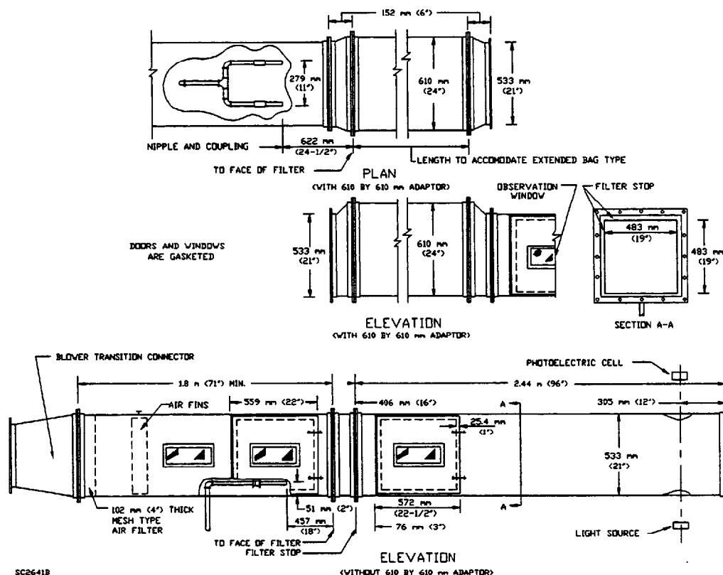
Figure 5.1 Flame exposure test apparatus
