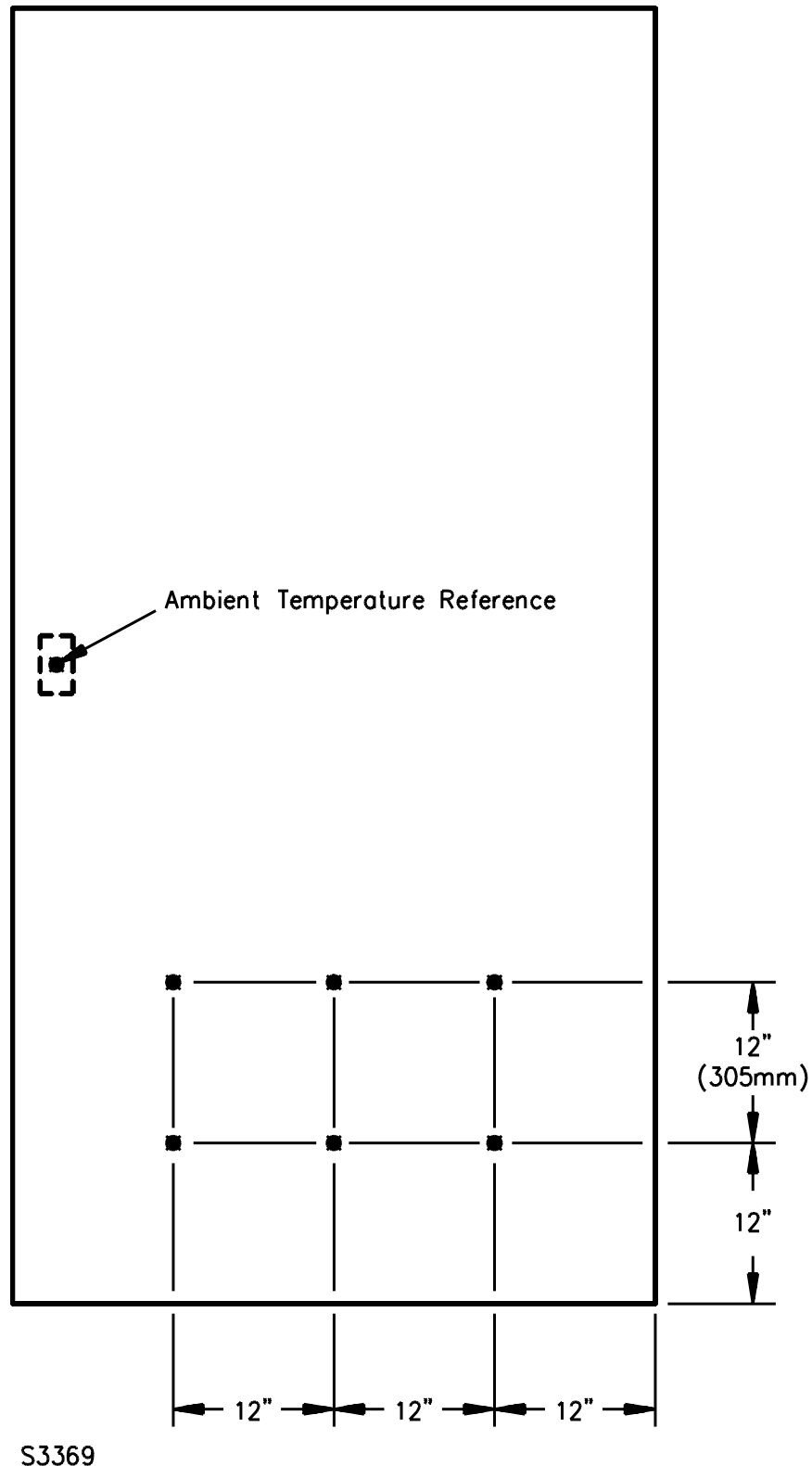
Figure 11.4 Thermocouple locations, left adjustable side wall
