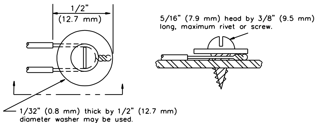
THERMOCOUPLE SECURED TO METAL SURFACES
