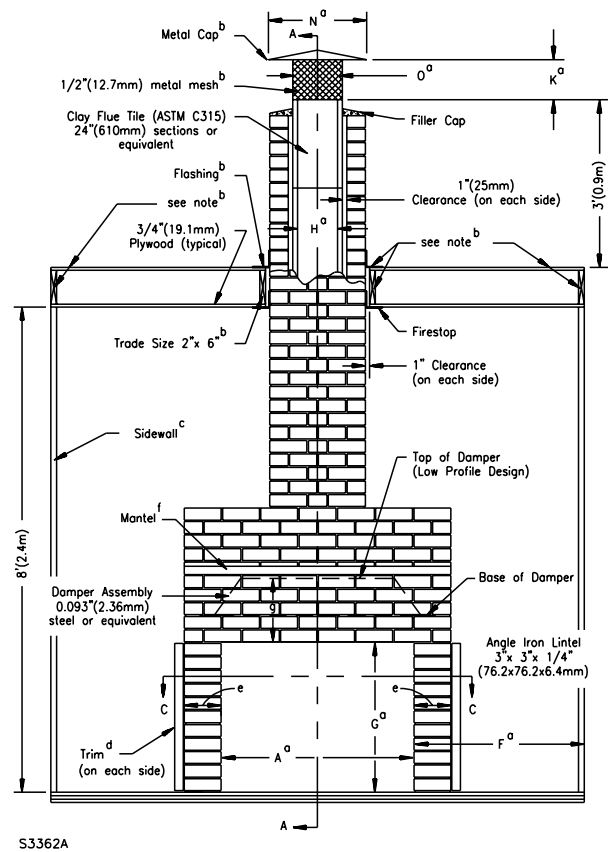
Figure 10.1 Masonry fireplace – front elevation
